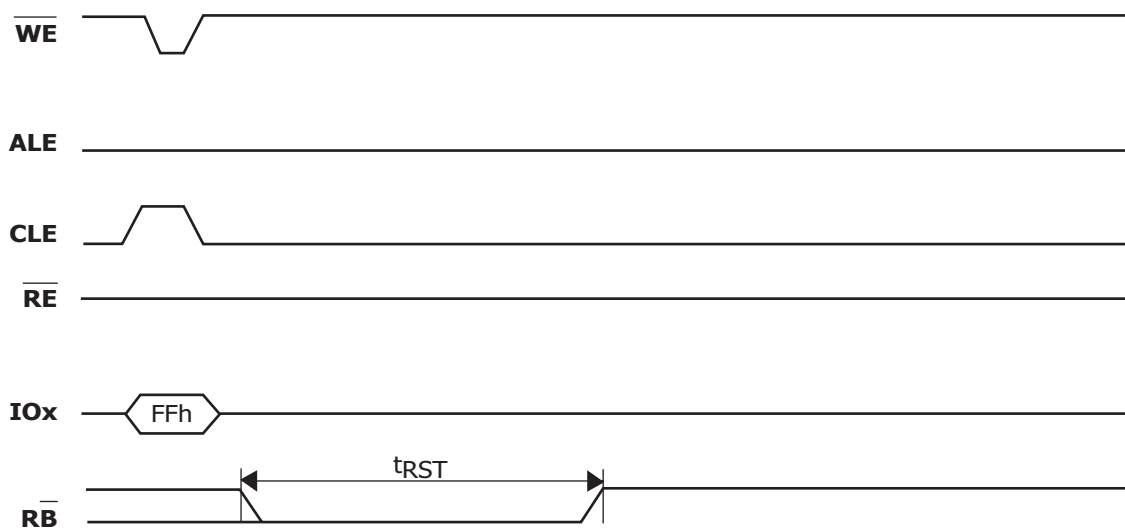
Figure 27: Reset Operation
